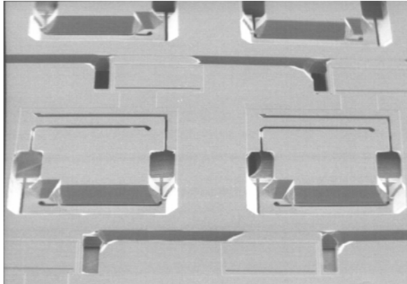
Spring mass system single crystalline Si
