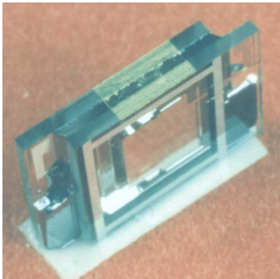
Complete Sensor chip, vertical mounted size (10 x 7 x 1,5) mm 3
