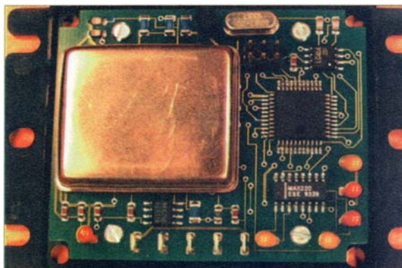
Inclination sensor system (hybrid)
