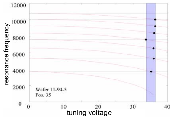
tuning curves
