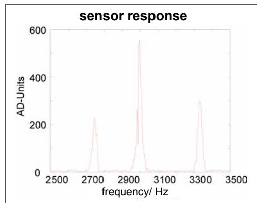
tuning curves
